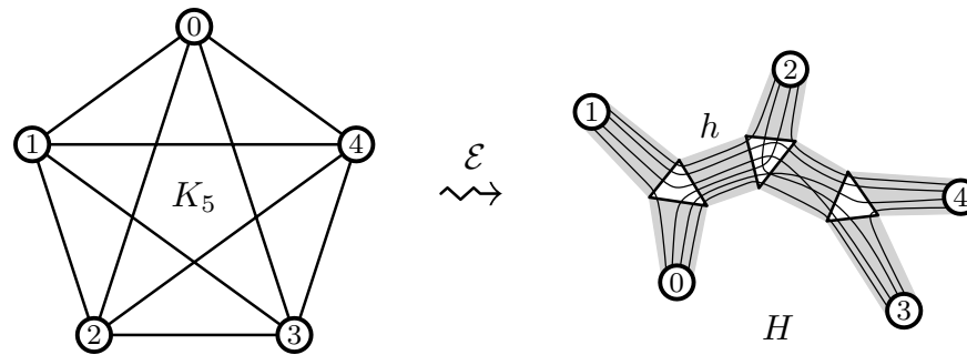
Figure 2: The complete graph K_5 (guest) routed along an unrooted binary tree H (host). We have \text{cng}_{H,\mathcal{E}}(K_5) = 6 which is witnessed by h : six arcs of K_5 are running parallel to h
